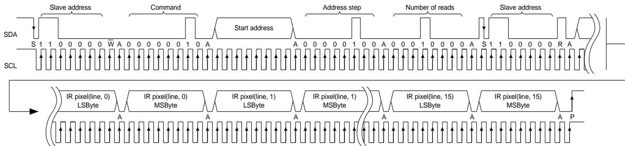
Figure 13 Single line (SA = 0x60, command = 0x02, Start address = 0x00...0x03 (step 0x01), Address step = 0x04, Number of reads = 0x10) measurement result read
