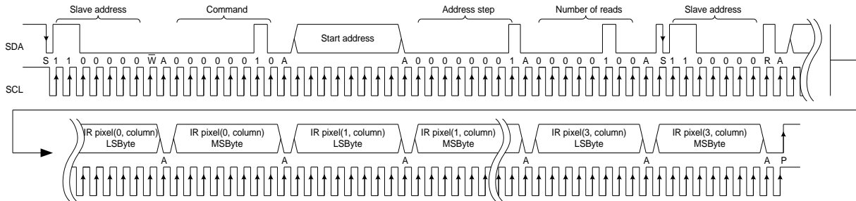
Figure 12 Single column (SA = 0x60, command = 0x02, Start address = 0x00...0x3C (step 0x04), Address step = 0x01, Number of reads = 0x04) measurement result read
