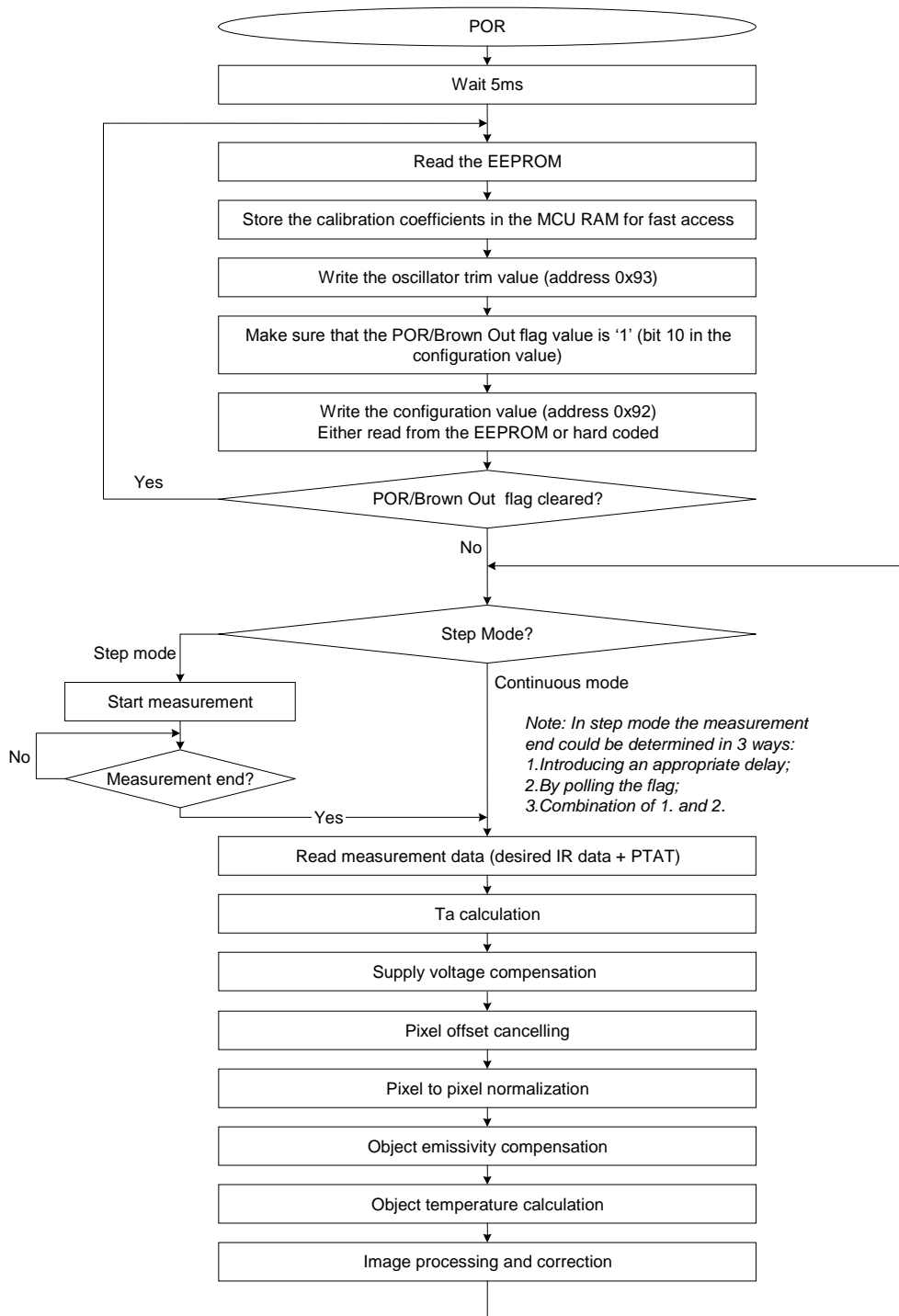
Figure 18: temperature calculation flow
